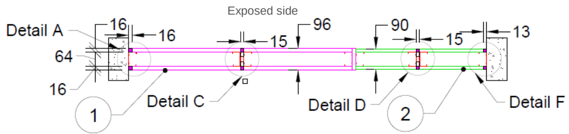
Figure 5 Cross-section C-C
