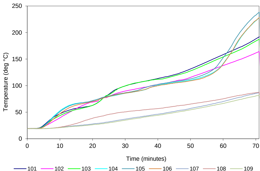
Figure 14 Control joint F – temperature vs time
