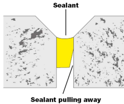
Incorrect: Sealant extends too deep into joint leading to tearing away from sides or splitting
