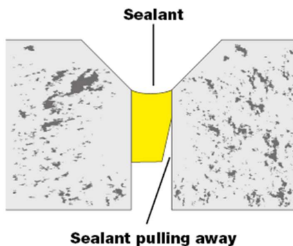
Incorrect: Sealant extends too deep into joint leading to tearing away from sides or splitting
