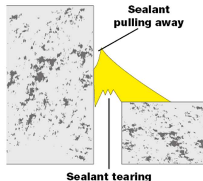
Incorrect: Sealant applied without backing rod or where excessive movement occurs, allows sealant to split away from the wall edges and tear
