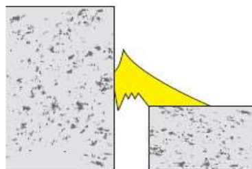
Incorrect: Sealant applied without backing rod or where excessive movement occurs, allows sealant to split away from the wall edges and tear
