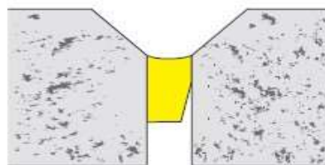
Incorrect: No backing rod and sealant extends too deep into joint leading to tearing away from sides or splitting
