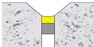
Correct: Sealant applied to joint with backing rod and correct sealant width:depth ratio
