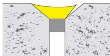
Incorrect: Sealant applied onto chamfered edge where concrete may be weak causing sealant to tear away
