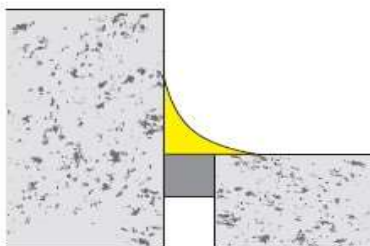
Correct: Sealant applied between two walls with backing rod to support movement
